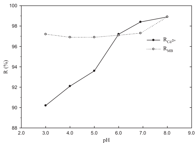
Fig. 6. Effect of pH values on removal efficiency of MB and Cd 2+ in simultaneous removal process.
