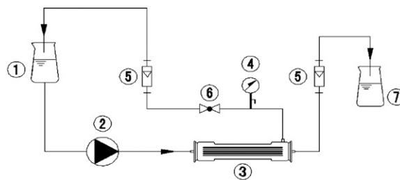
Fig. 1. Schematic diagram of ultrafiltration system: (1) feed tank, (2) peristaltic pump, (3) membrane, (4) manometer, (5) rotameter, (6) pressure control valve, (7) permeate tank.
