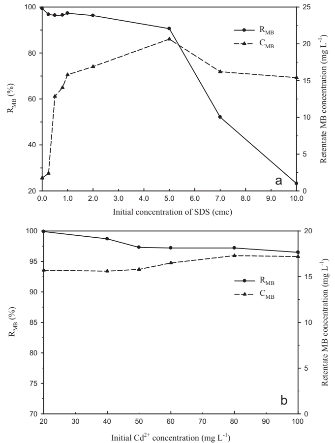
Fig. 5. Effects of initial SDS (a) and Cd^{2+} (b) concentrations on removal efficiency and retentate concentration of MB in simultaneous removal process.
