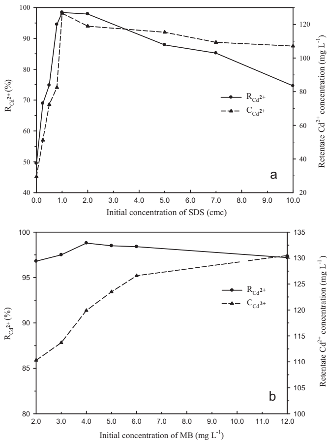
Fig. 4. Effects of initial SDS (a) and MB (b) concentrations on removal efficiency and retentate concentration of Cd^{2+} in simultaneous removal process.
